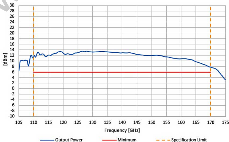
Power vs Frequency
