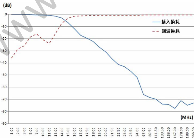
插入损耗及回波损耗测试曲线 Insertion Loss & Return Loss Test Curve
