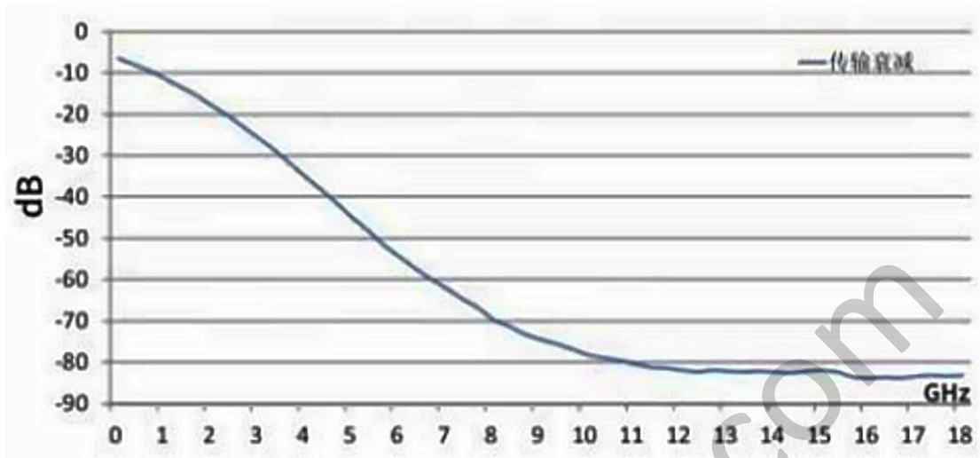
传输衰减测试曲线 Attenuation Test Curve
