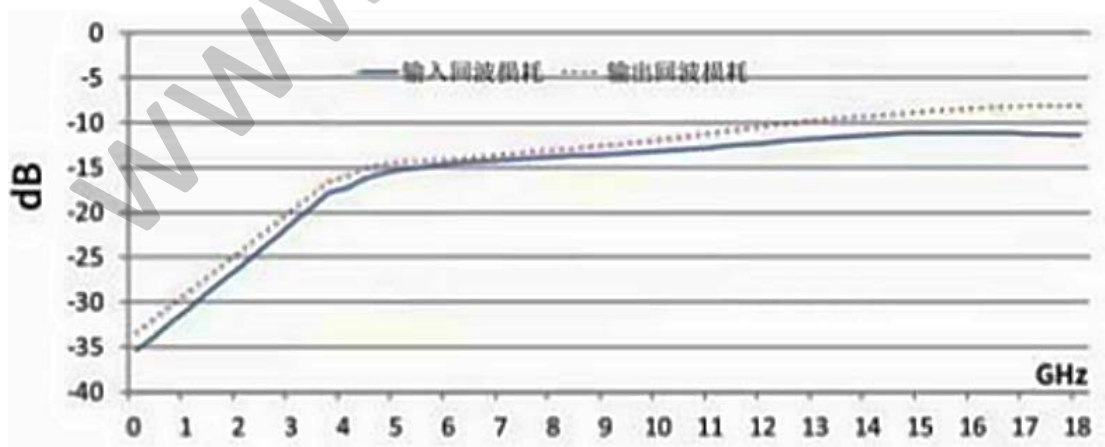
回波损耗测试曲线 Return Loss Test Curve
