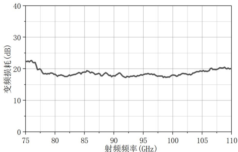
Conversion Loss vs Frequency
