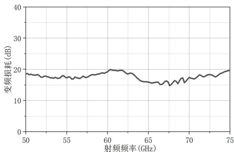
Conversion Loss vs Frequency
