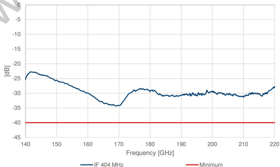
Conversion Loss(SSB) vs Frequency
