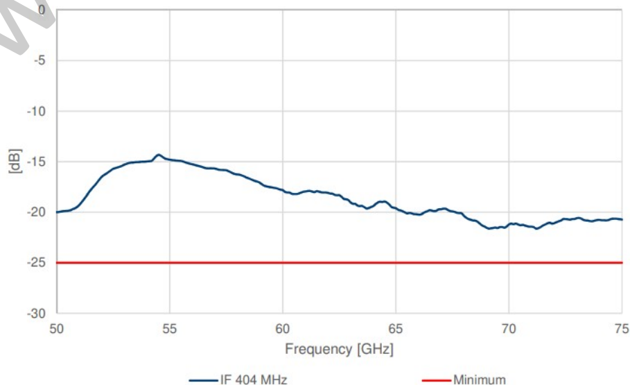
Conversion Loss(SSB) vs Frequency
