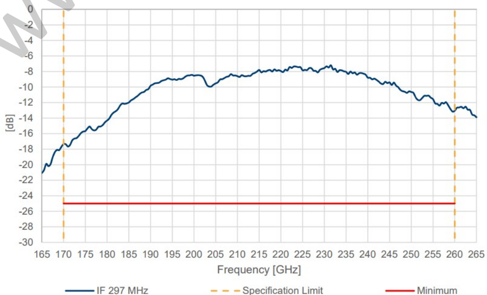
Conversion Loss(SSB) vs Frequency
